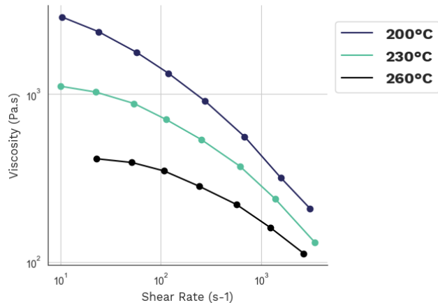
Viscosity-shear rate Pebax® 7233 SP 01
