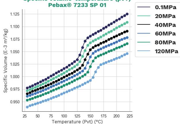
Specific volume-temperature (pvT) Pebax® 7233 SP 01
